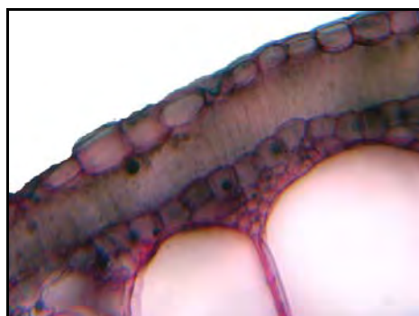
Figure 3. Micrograph of cross section through the lamina of Petrosimonia triandra (X400).
