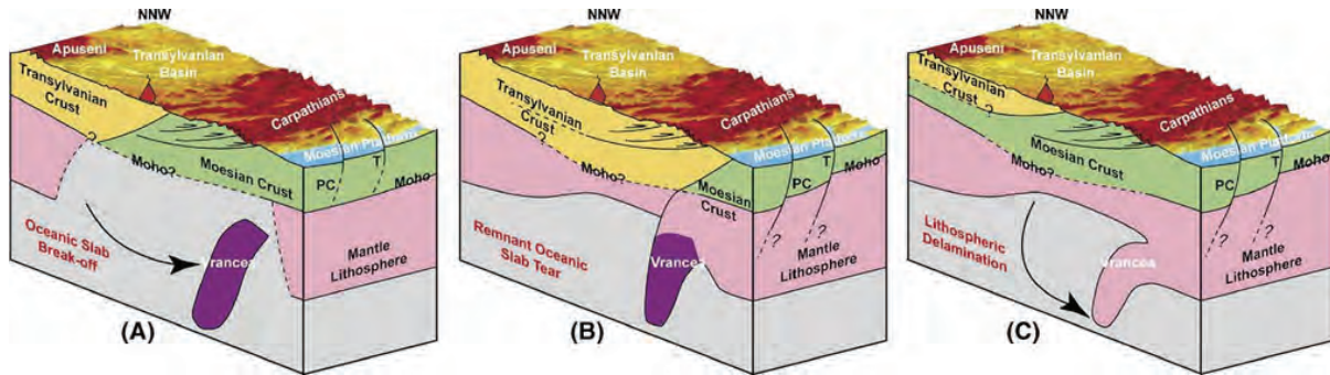
Figure 2. The main geodynamic scenarios are: (A) the subduction of an ocean plate and its break-off, (B) the subduction of an ocean plate, and (C) progressive lateral tearing under the Carpathian vortex and delamination of the continental lithosphere (after KNAPP et al., 2005)
